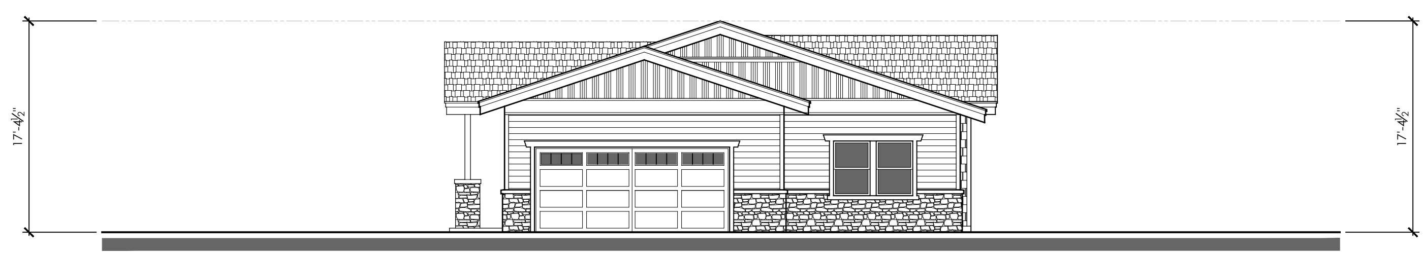
3 BUILDING 5 SOUTH ELEVATION 1/8" = 1'-0"
