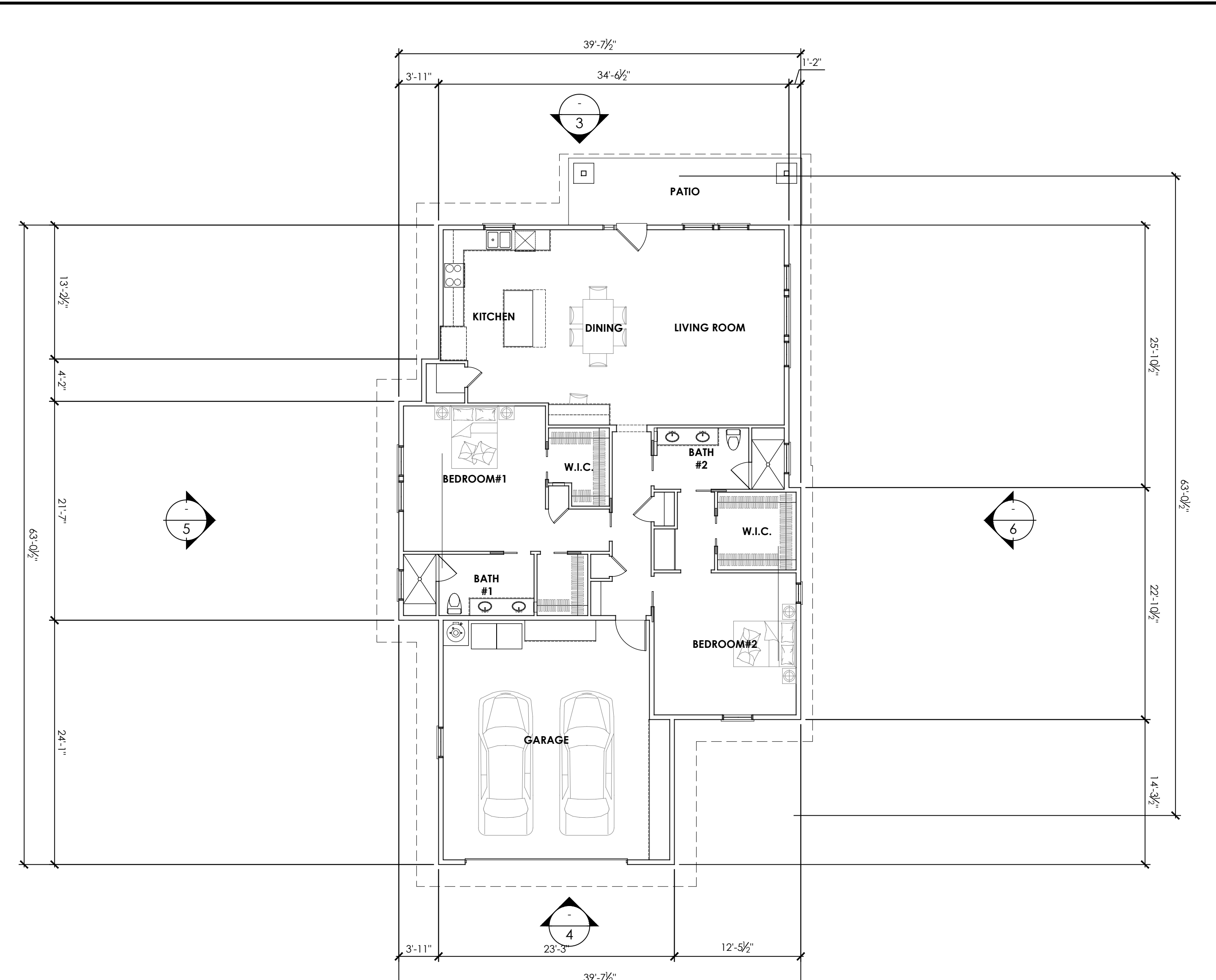
1 BUILDING 6 FLOOR PLAN 1/8" = 1'-0"
