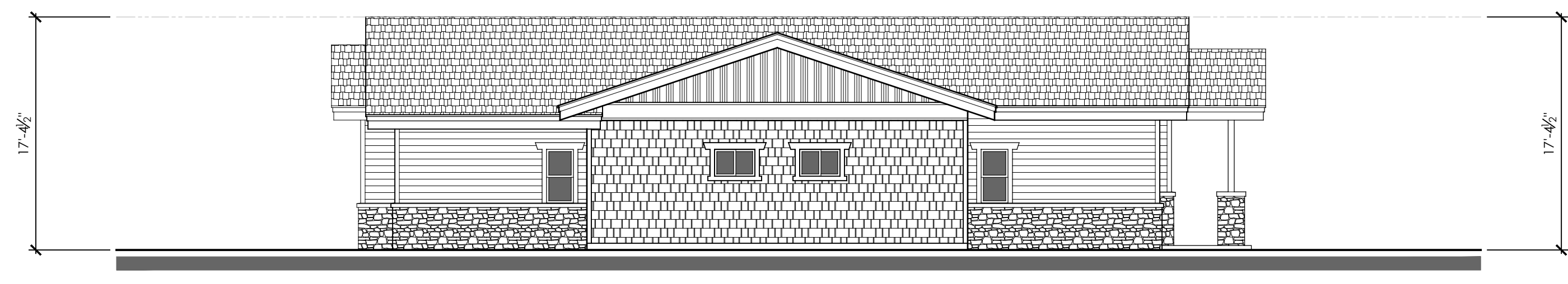
6 BUILDING 5 EAST ELEVATION 1/8" = 1'-0"
