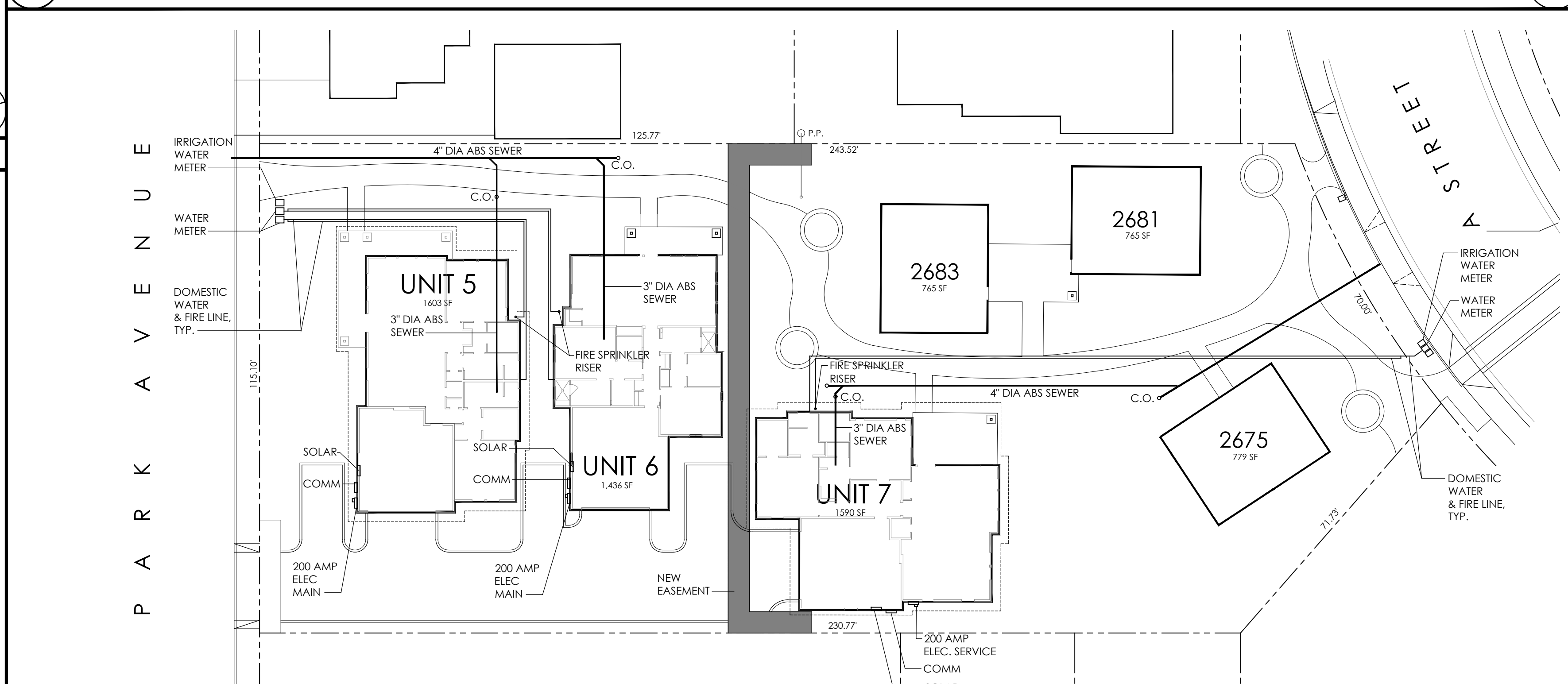
1 ENLARGED SITE PLAN/ CONCEPT FIRE SPRINKLER RISER PLAN - NORTH LOT 1"=20'-0"
